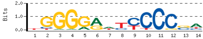
primary_MA0105_extended
