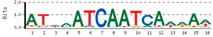
primary_MA0070_extended
