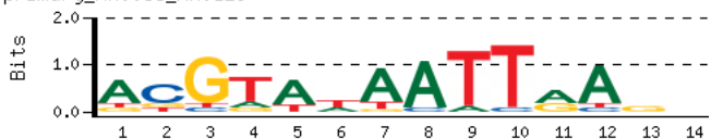
primary_MA0063_MA0129
