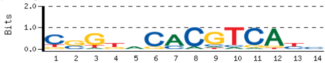
primary_MA0097_extended
