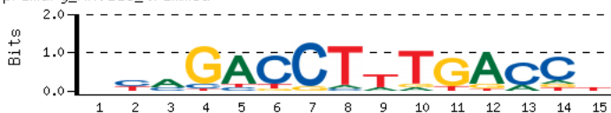
primary_MA0115_trimmed
