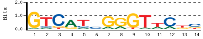
primary_MA0074_trimmed
