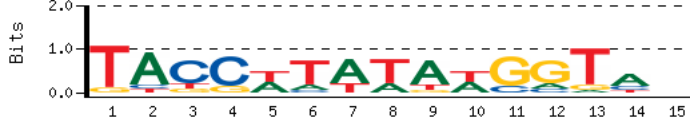
primary_MA0083_extended
