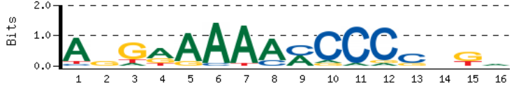
primary_MA0022_extended
