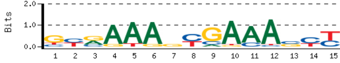
primary_MA0050_extended
